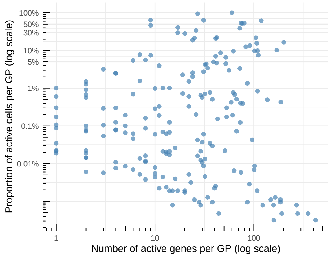
Active genes vs. active-cell proportion per GP
